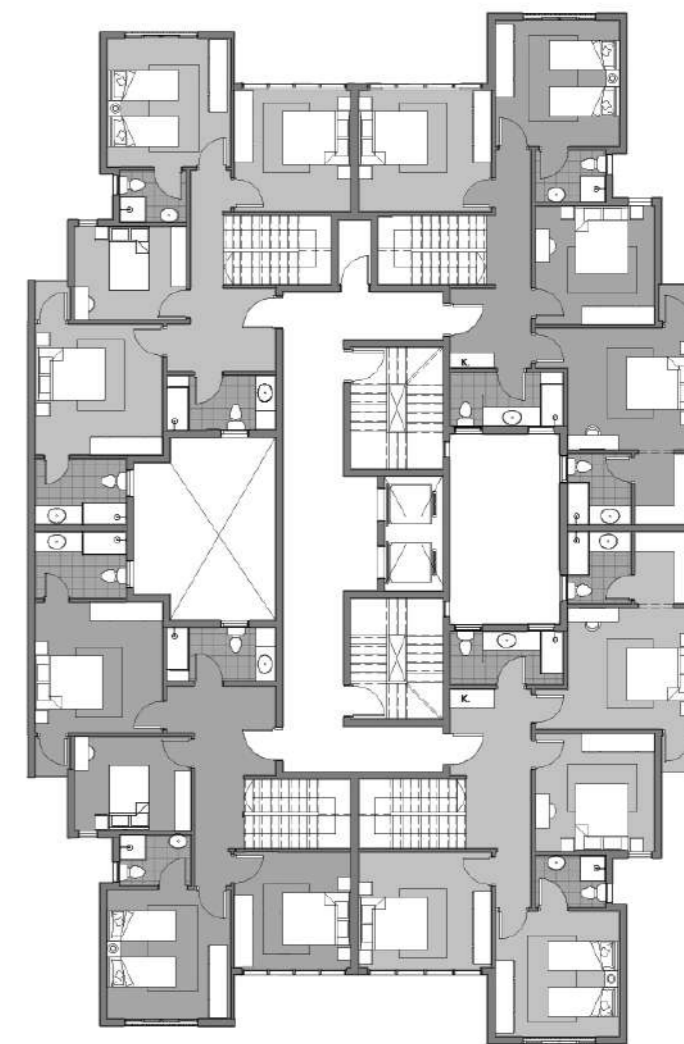
SEVENTH FLOOR PLAN
