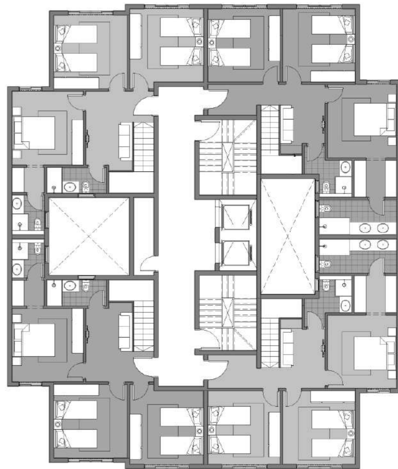
FIFTH FLOOR PLAN
