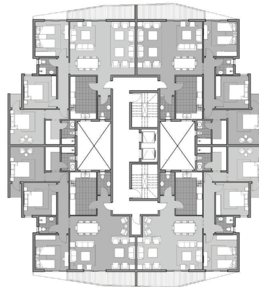
SIXTH FLOOR PLAN
